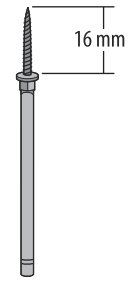
CASPAR WIS-FF-205 70 mm
